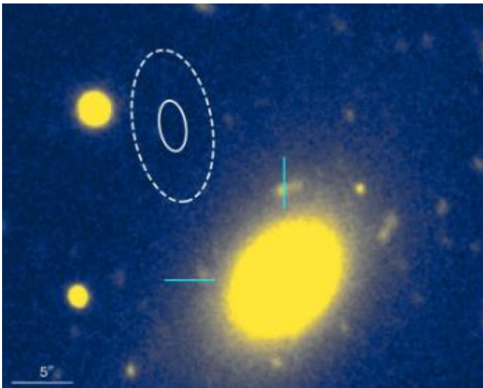
The location of the fast radio burst, indicated by the oval outlines, is on the outskirts of a massive elliptical galaxy, the yellow oval at right. Gemini Observatory
